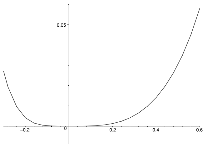
Figure 1. The functions V(\xi) for c_1 = 0 and c_1 = 0.5 .
